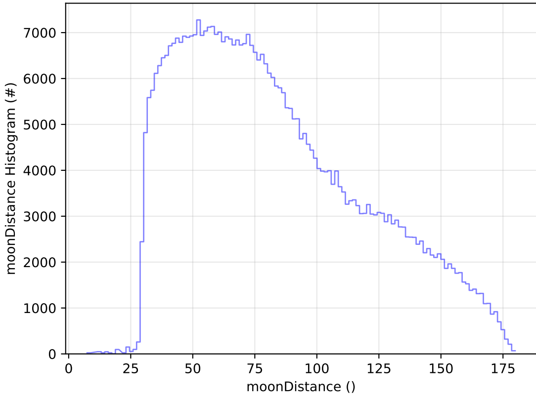
ddf_acor_sf20_lsf40_lsr50_v3.4_10yrs All sky z band: moonDistance Histogram
