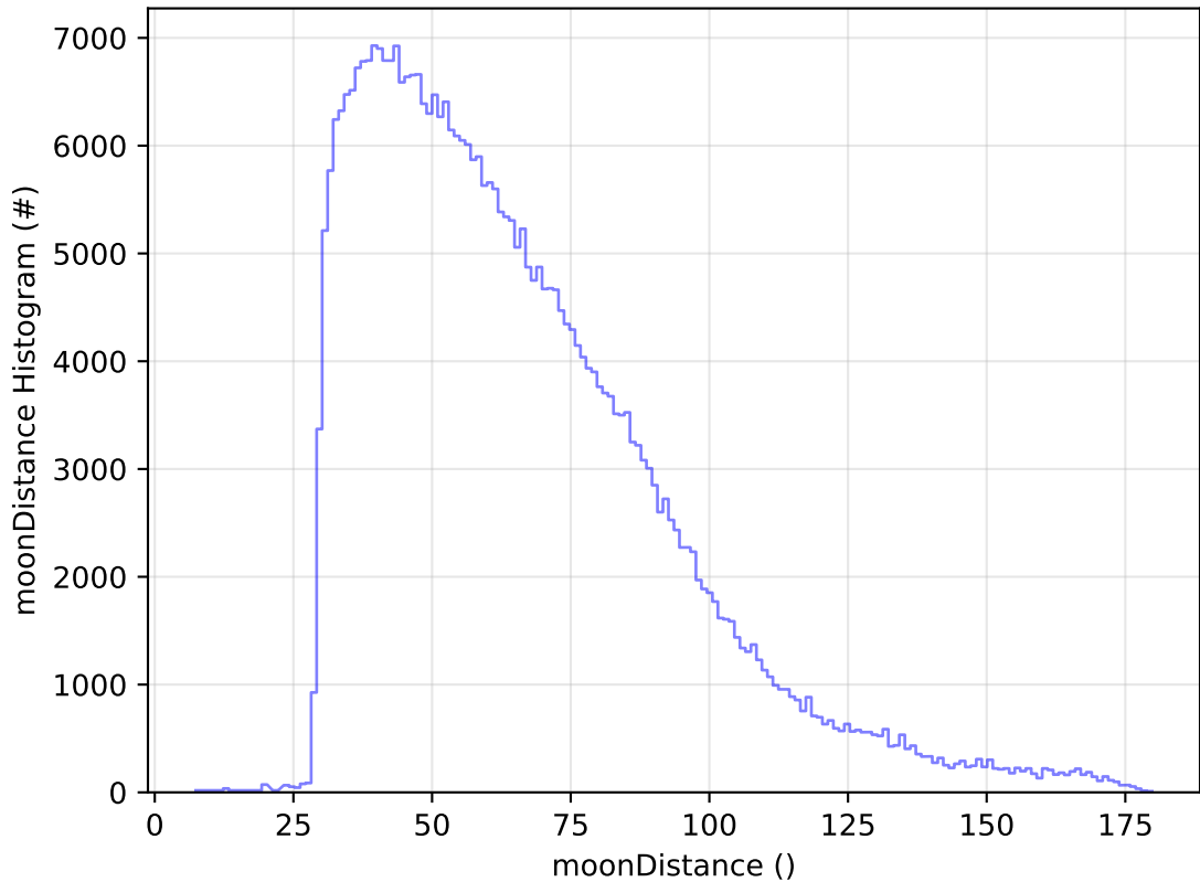
ddf_acor_sf20_lsf40_lsr50_v3.4_10yrs All sky y band: moonDistance Histogram
