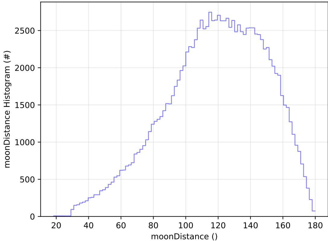
ddf_acor_sf20_lsf40_lsr50_v3.4_10yrs All sky u band: moonDistance Histogram
