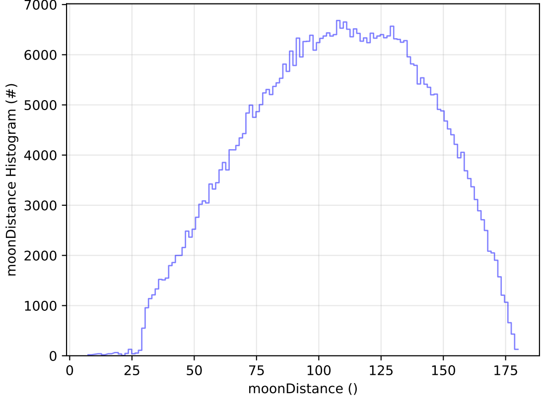
ddf_acor_sf20_lsf40_lsr50_v3.4_10yrs All sky r band: moonDistance Histogram
