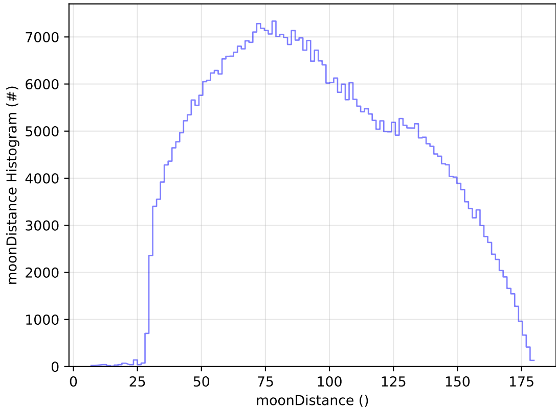
ddf_acor_sf20_lsf40_lsr50_v3.4_10yrs All sky i band: moonDistance Histogram
