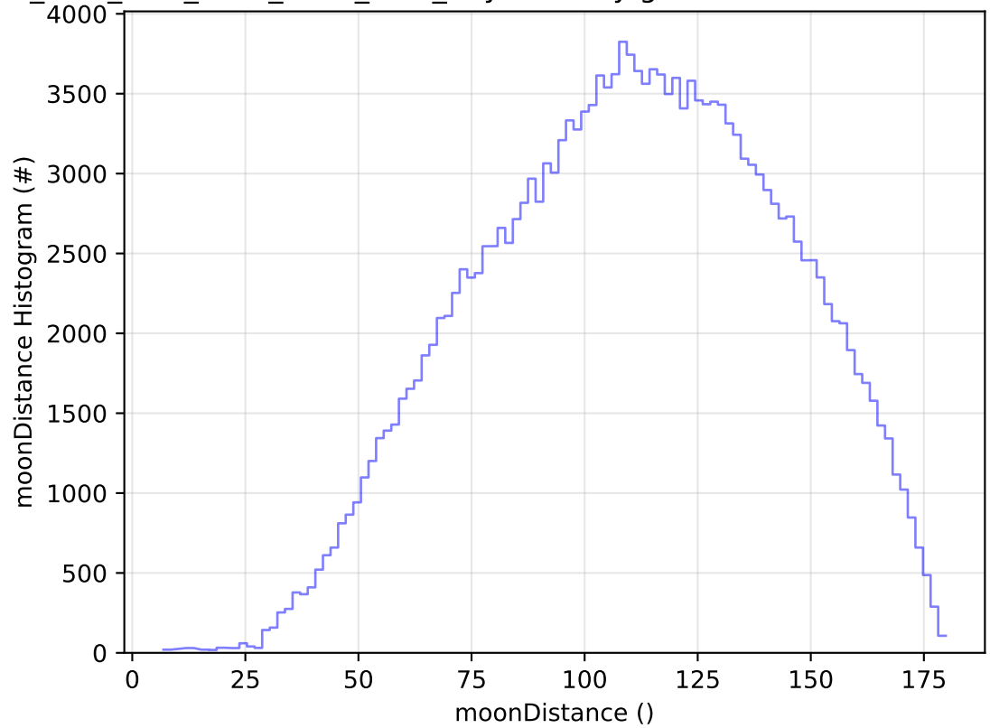
ddf_acor_sf20_lsf40_lsr50_v3.4_10yrs All sky g band: moonDistance Histogram
