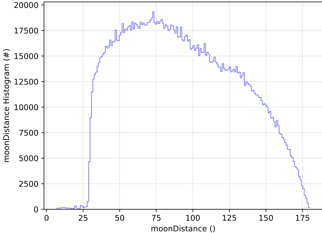
ddf_acor_sf20_lsf40_lsr50_v3.4_10yrs All sky all bands: moonDistance Histogram
