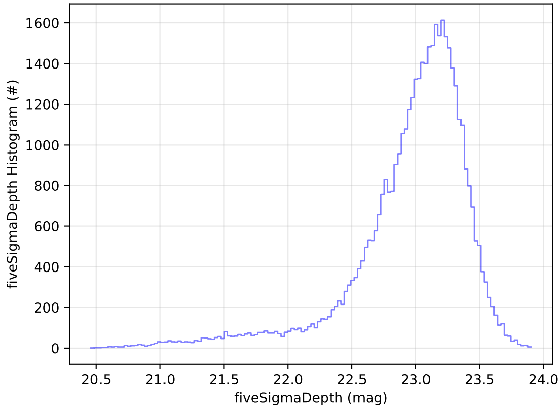
ddf_acor_sf20_lsf40_lsr50_v3.4_10yrs Yr 1 z band: fiveSigmaDepth Histogram
