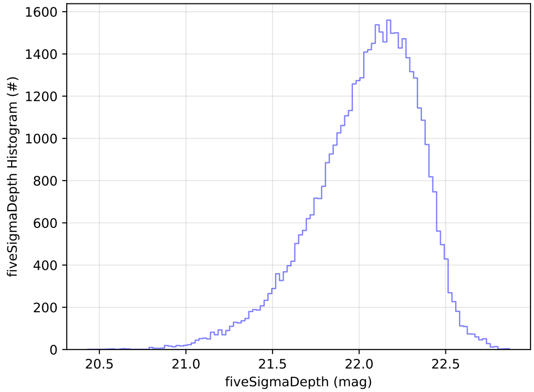
ddf_acor_sf20_lsf40_lsr50_v3.4_10yrs Yr 1 y band: fiveSigmaDepth Histogram
