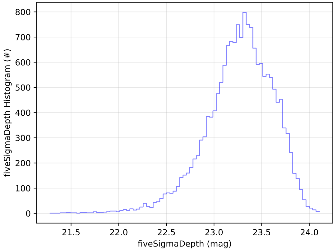
ddf_acor_sf20_lsf40_lsr50_v3.4_10yrs Yr 1 u band: fiveSigmaDepth Histogram
