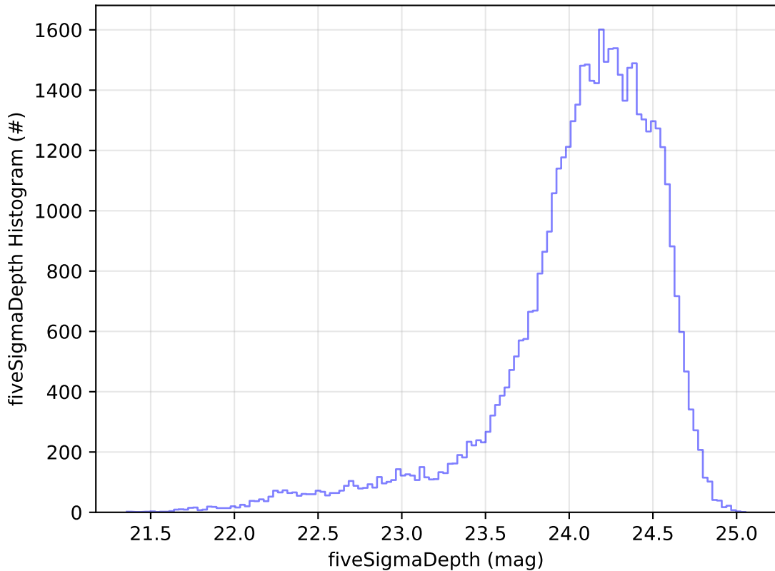
ddf_acor_sf20_lsf40_lsr50_v3.4_10yrs Yr 1 r band: fiveSigmaDepth Histogram
