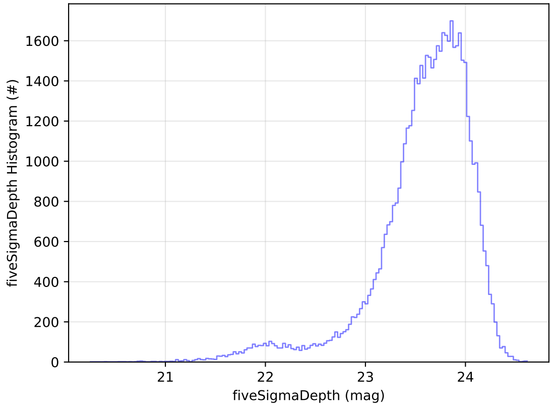
ddf_acor_sf20_lsf40_lsr50_v3.4_10yrs Yr 1 i band: fiveSigmaDepth Histogram
