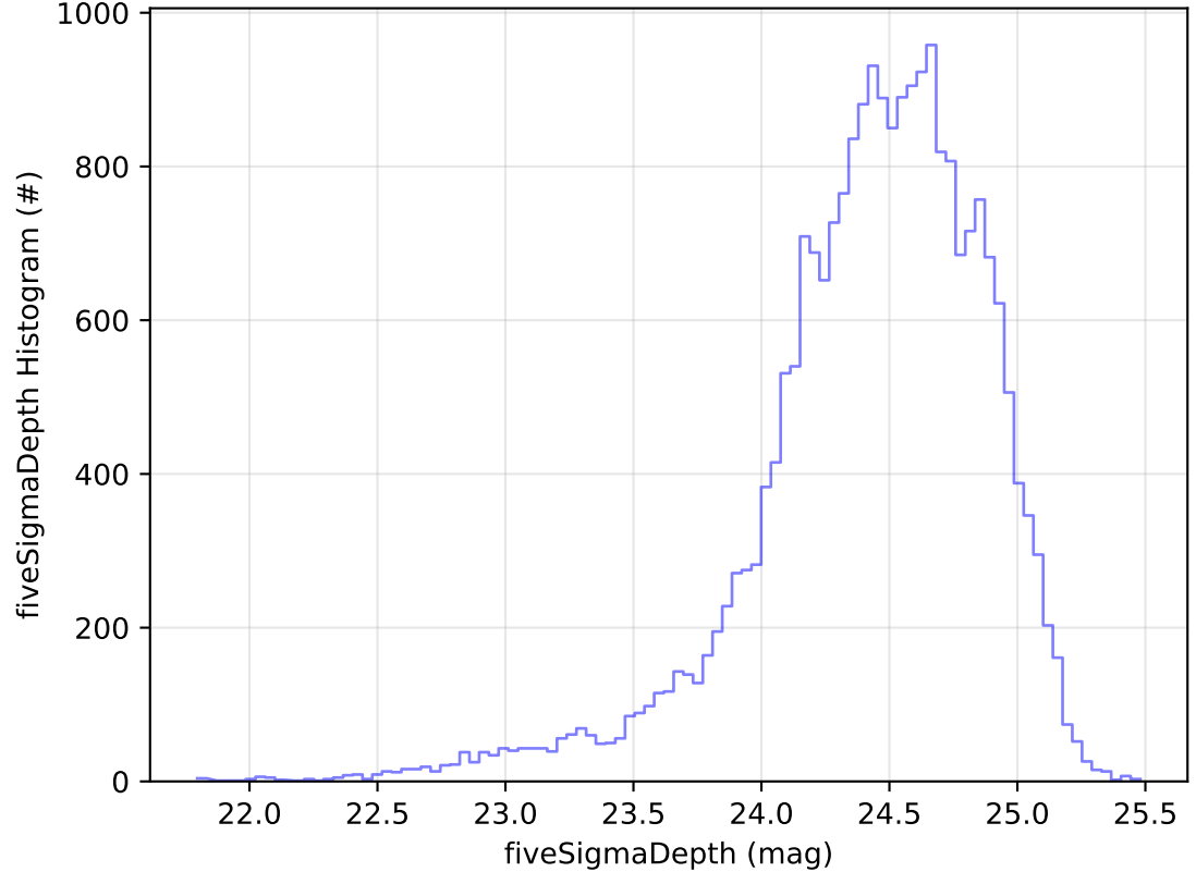
ddf_acor_sf20_lsf40_lsr50_v3.4_10yrs Yr 1 g band: fiveSigmaDepth Histogram
