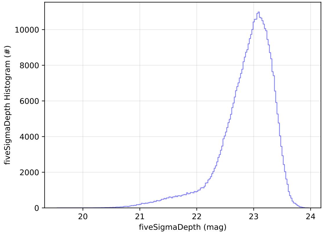
ddf_acor_sf20_lsf40_lsr50_v3.4_10yrs WFD z band: fiveSigmaDepth Histogram
