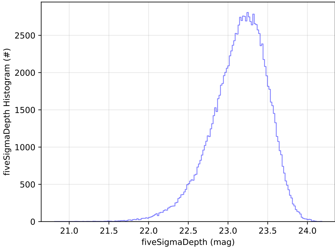
ddf_acor_sf20_lsf40_lsr50_v3.4_10yrs WFD u band: fiveSigmaDepth Histogram
