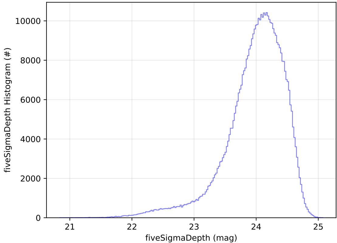
ddf_acor_sf20_lsf40_lsr50_v3.4_10yrs WFD r band: fiveSigmaDepth Histogram
