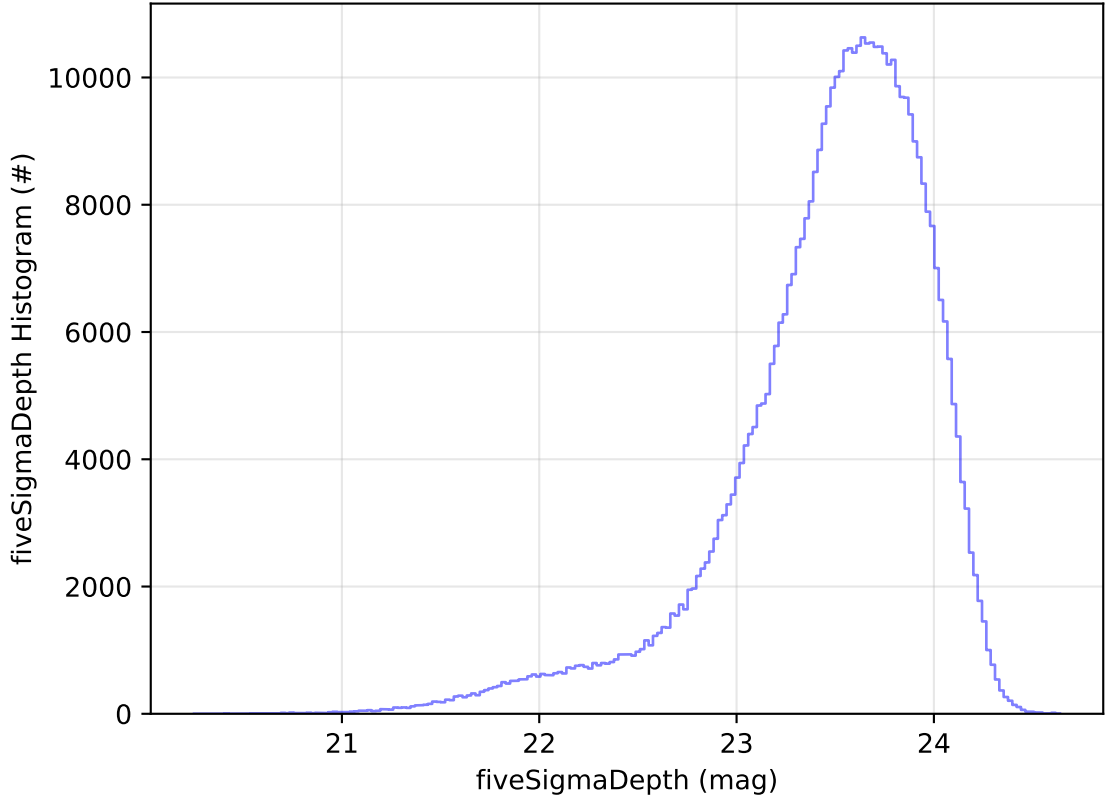
ddf_acor_sf20_lsf40_lsr50_v3.4_10yrs WFD i band: fiveSigmaDepth Histogram
