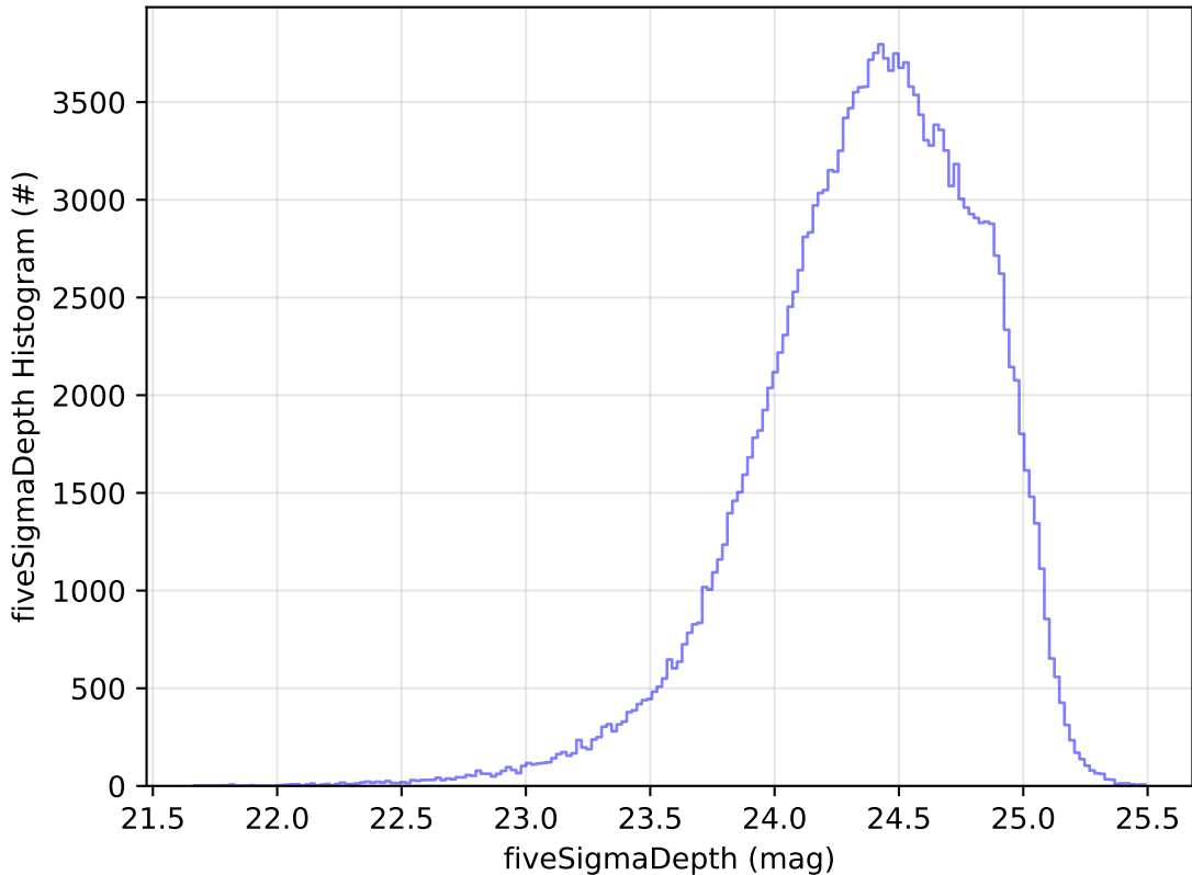
ddf_acor_sf20_lsf40_lsr50_v3.4_10yrs WFD g band: fiveSigmaDepth Histogram
