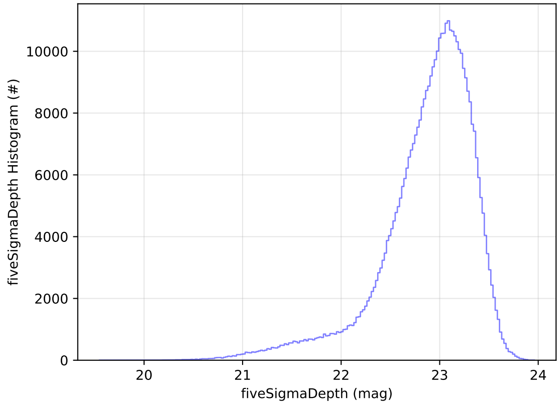
ddf_acor_sf20_lsf40_lsr50_v3.4_10yrs All sky z band: fiveSigmaDepth Histogram
