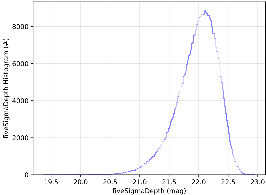
ddf_acor_sf20_lsf40_lsr50_v3.4_10yrs All sky y band: fiveSigmaDepth Histogram
