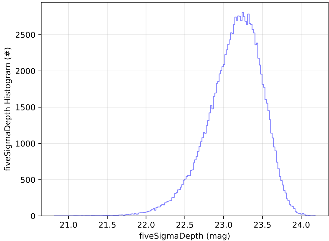
ddf_acor_sf20_lsf40_lsr50_v3.4_10yrs All sky u band: fiveSigmaDepth Histogram
