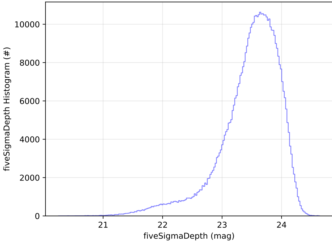
ddf_acor_sf20_lsf40_lsr50_v3.4_10yrs All sky i band: fiveSigmaDepth Histogram
