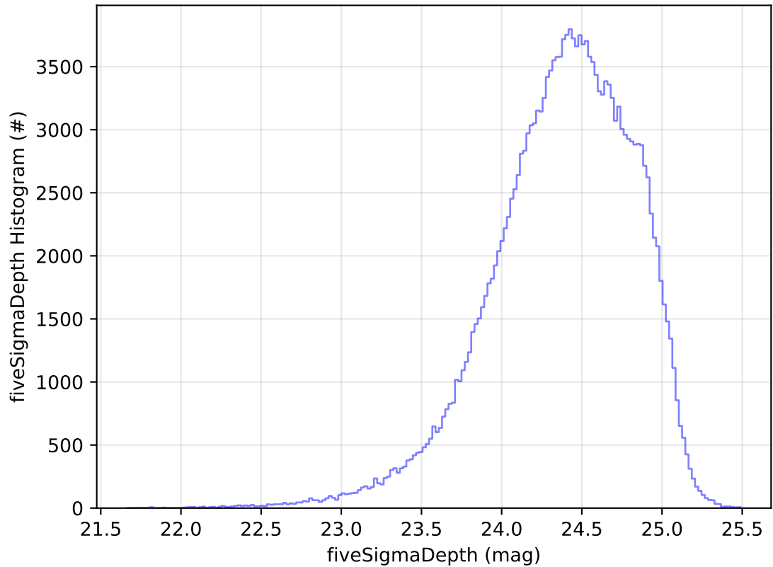
ddf_acor_sf20_lsf40_lsr50_v3.4_10yrs All sky g band: fiveSigmaDepth Histogram
