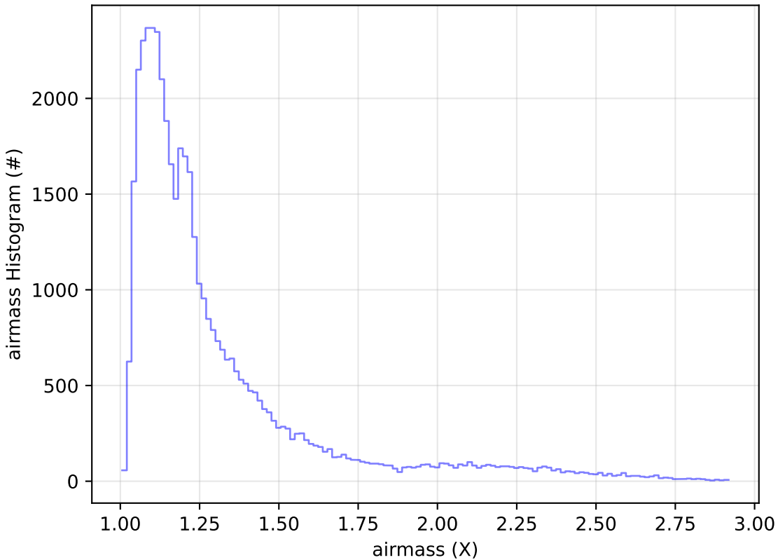
ddf_acor_sf20_lsf40_lsr50_v3.4_10yrs Yr 1 z band: airmass Histogram
