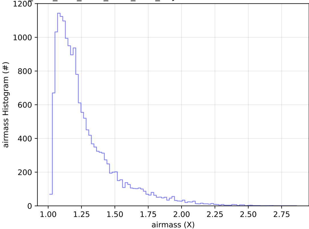
ddf_acor_sf20_lsf40_lsr50_v3.4_10yrs Yr 1 u band: airmass Histogram
