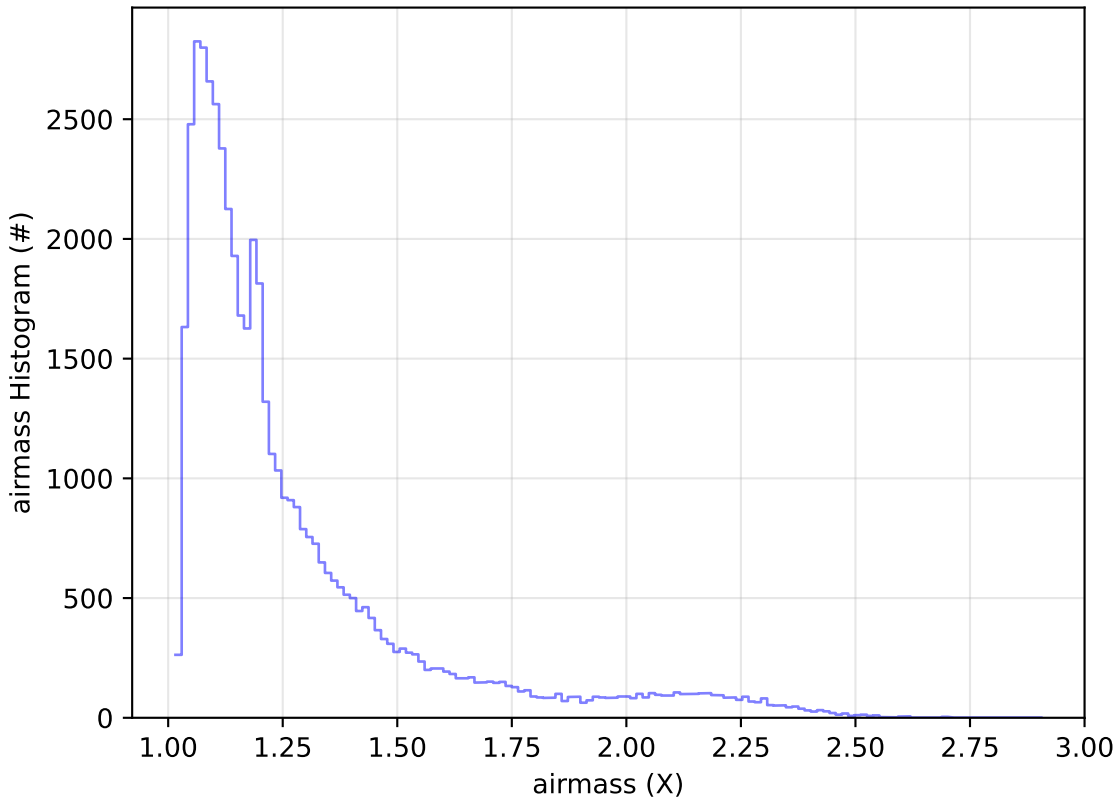
ddf_acor_sf20_lsf40_lsr50_v3.4_10yrs Yr 1 r band: airmass Histogram
