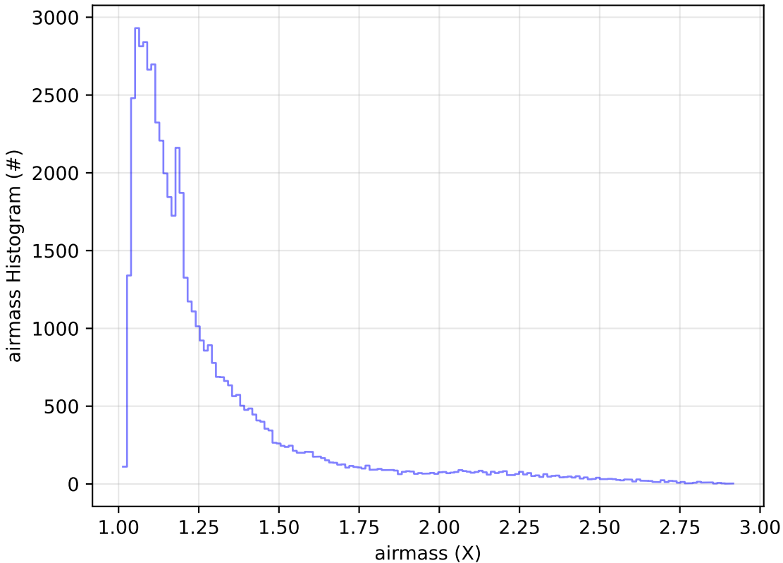
ddf_acor_sf20_lsf40_lsr50_v3.4_10yrs Yr 1 i band: airmass Histogram
