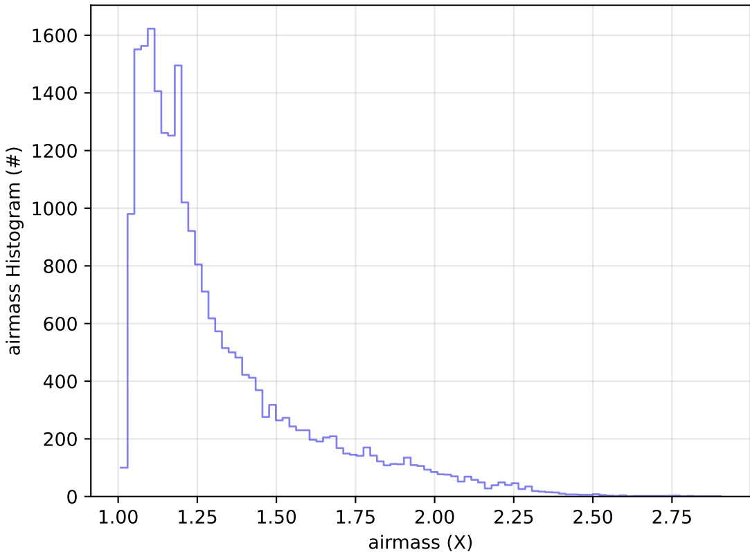
ddf_acor_sf20_lsf40_lsr50_v3.4_10yrs Yr 1 g band: airmass Histogram
