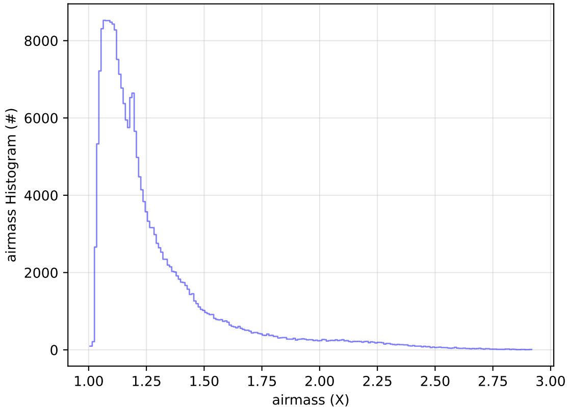
ddf_acor_sf20_lsf40_lsr50_v3.4_10yrs Yr 1 all bands: airmass Histogram
