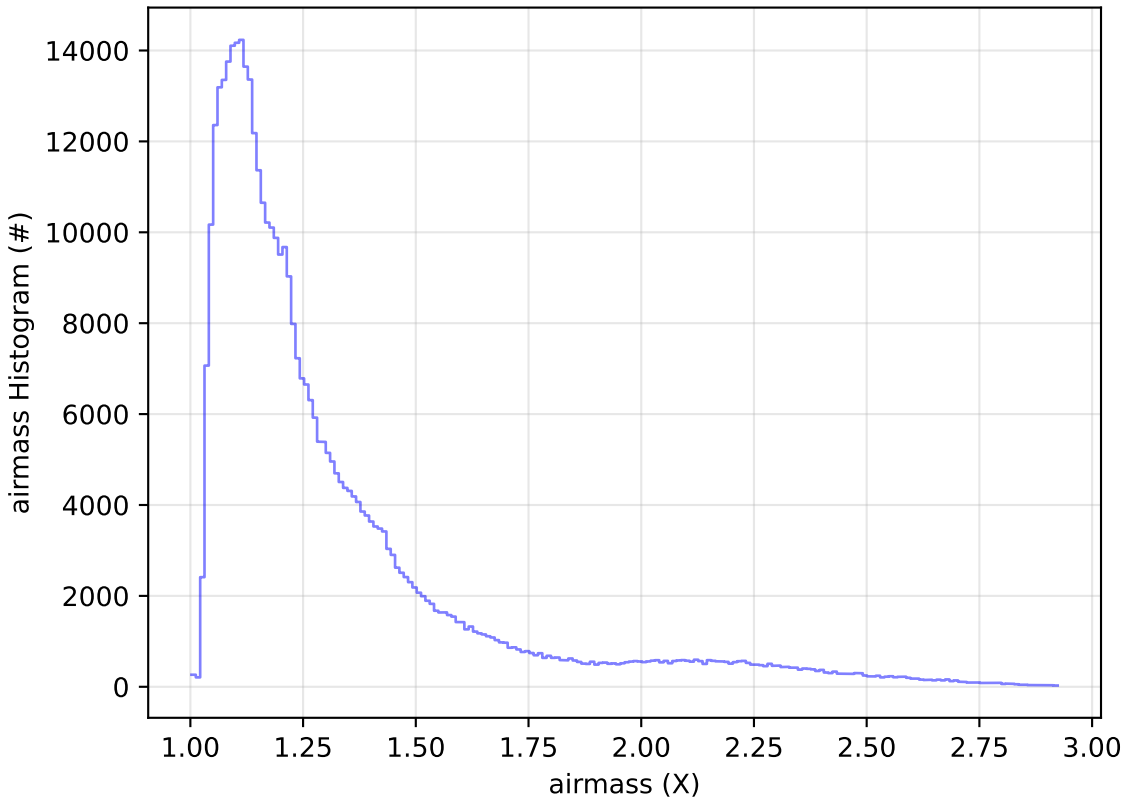
ddf_acor_sf20_lsf40_lsr50_v3.4_10yrs WFD z band: airmass Histogram
