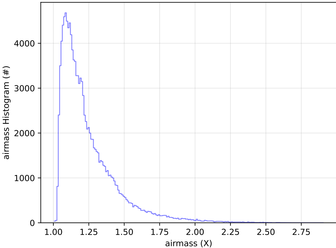
ddf_acor_sf20_lsf40_lsr50_v3.4_10yrs WFD u band: airmass Histogram
