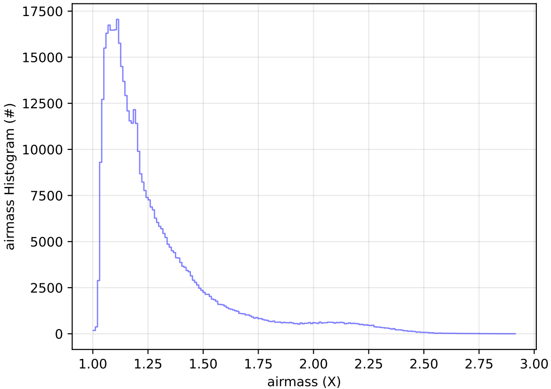
ddf_acor_sf20_Isf40_Isr50_v3.4_10yrs WFD r band: airmass Histogram
