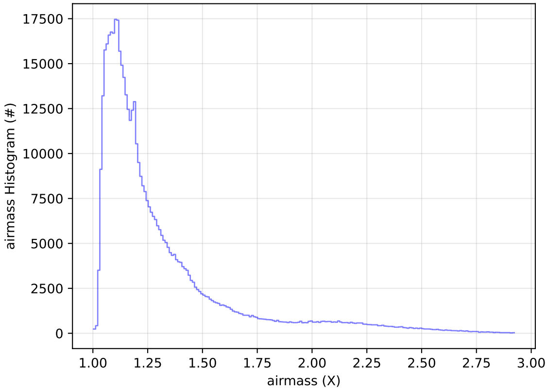
ddf_acor_sf20_lsf40_lsr50_v3.4_10yrs WFD i band: airmass Histogram
