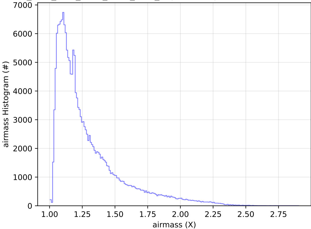
ddf_acor_sf20_lsf40_lsr50_v3.4_10yrs WFD g band: airmass Histogram
