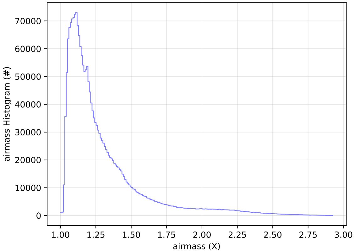
ddf_acor_sf20_lsf40_lsr50_v3.4_10yrs WFD all bands: airmass Histogram
