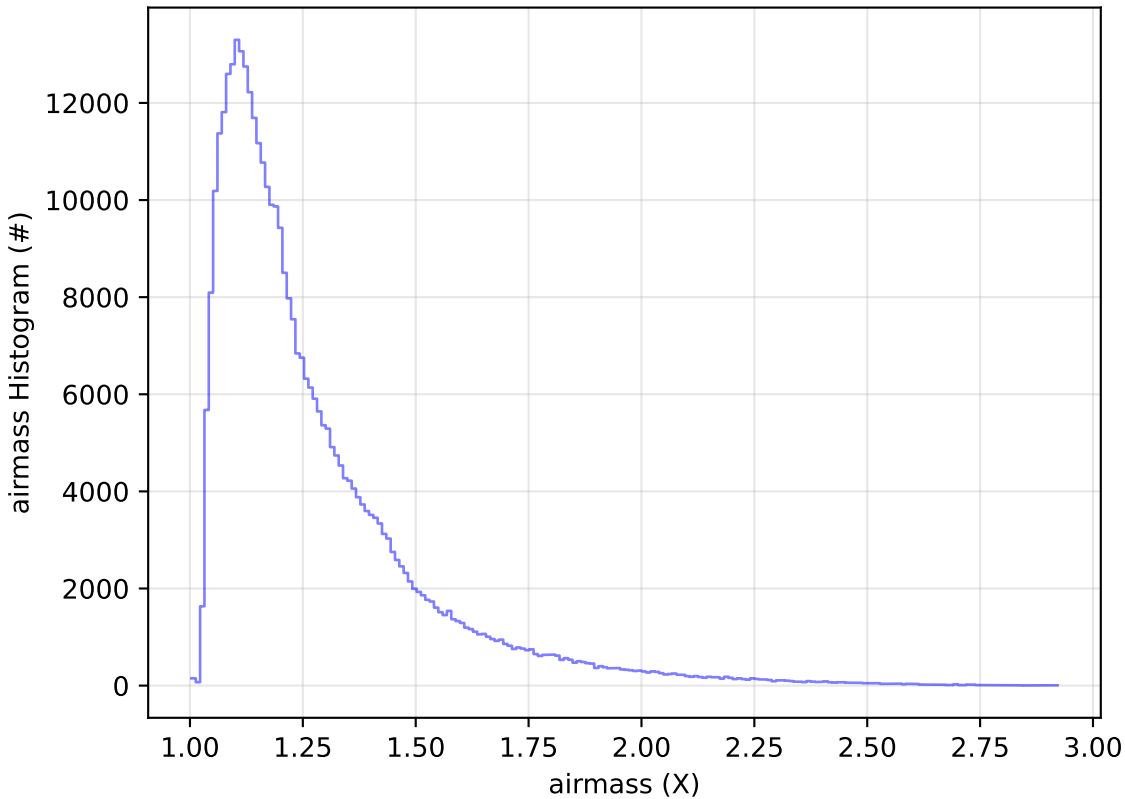
ddf_acor_sf20_lsf40_lsr50_v3.4_10yrs All sky y band: airmass Histogram
