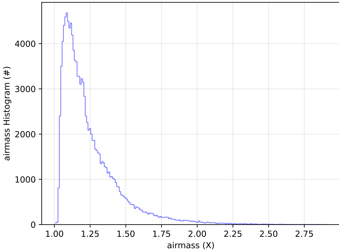
ddf_acor_sf20_lsf40_lsr50_v3.4_10yrs All sky u band: airmass Histogram
