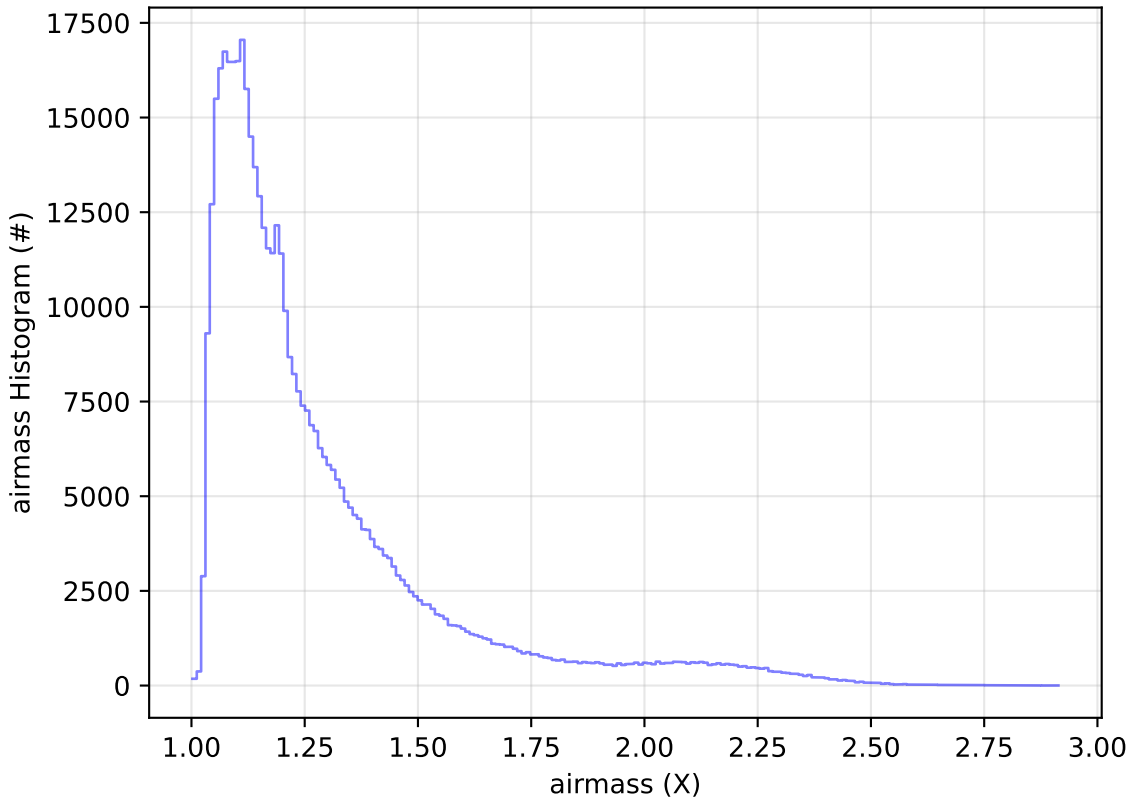
ddf_acor_sf20_lsf40_lsr50_v3.4_10yrs All sky r band: airmass Histogram
