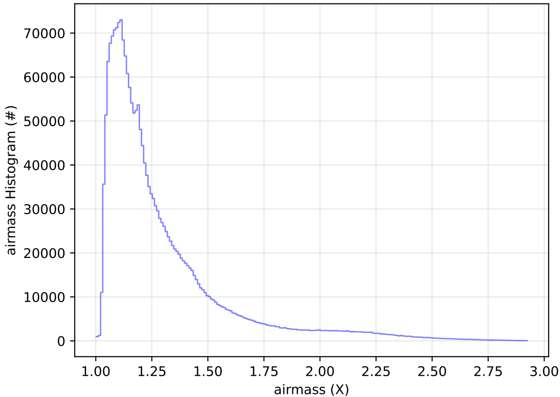
ddf_acor_sf20_lsf40_lsr50_v3.4_10yrs All sky all bands: airmass Histogram
