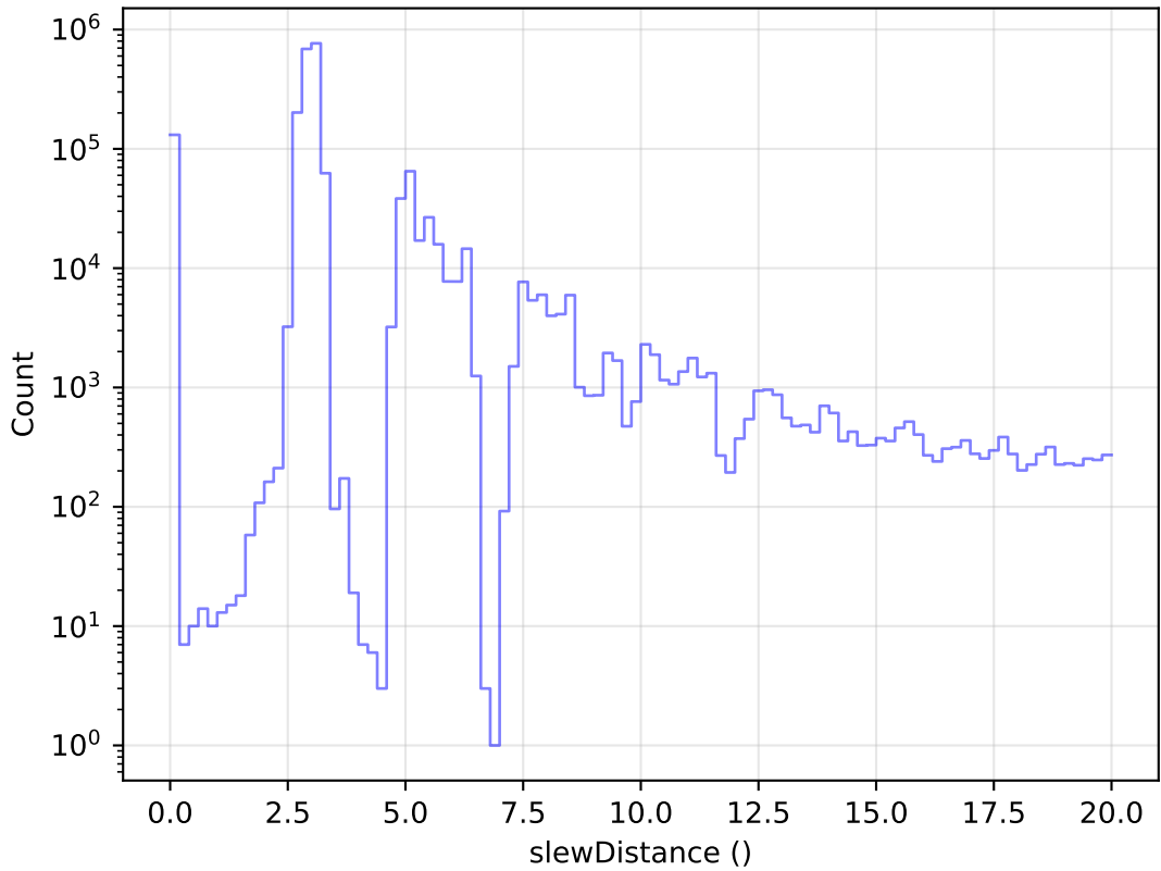
ddf_acor_sf20_lsf40_lsr50_v3.4_10yrs All visits: Zoom Slew Distance Histogram
