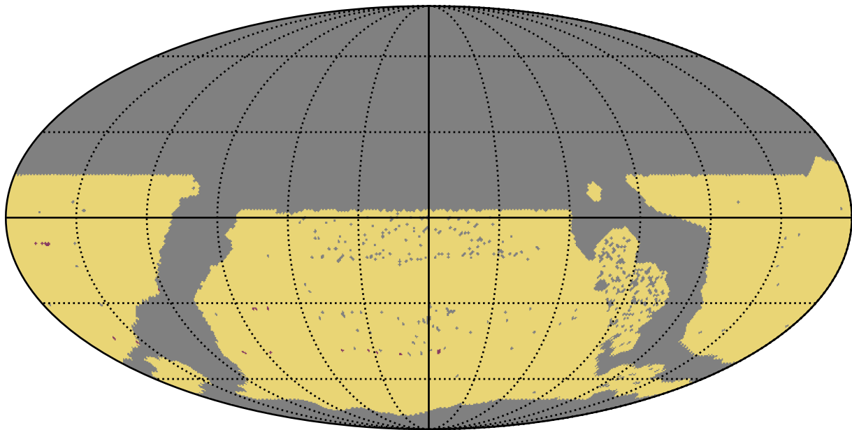
ddf_acor_sf20_lsf40_lsr50_v3.4_10yrs WFD: RapidRevisits
