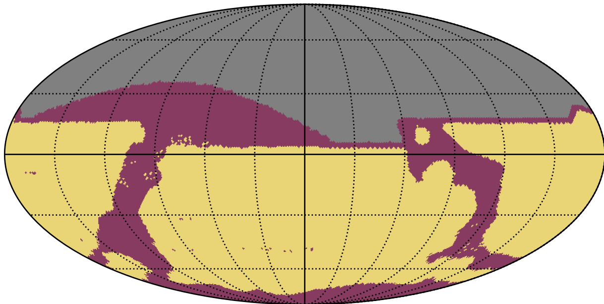
ddf_acor_sf20_lsf40_lsr50_v3.4_10yrs All sky: RapidRevisits
