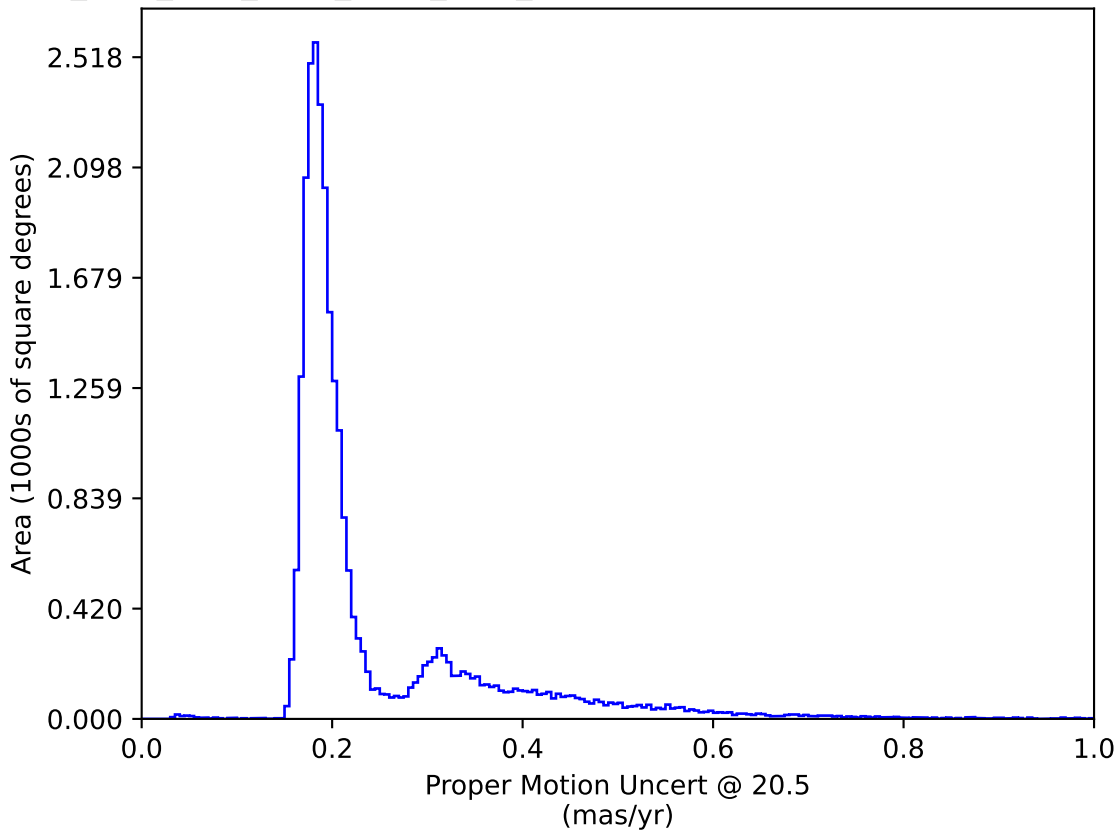
ddf_acor_sf20_lsf40_lsr50_v3.4_10yrs All sky: Proper Motion Uncert @ 20.5
