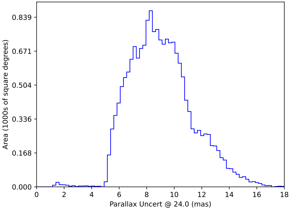
ddf_acor_sf20_lsf40_lsr50_v3.4_10yrs WFD: Parallax Uncert @ 24.0
