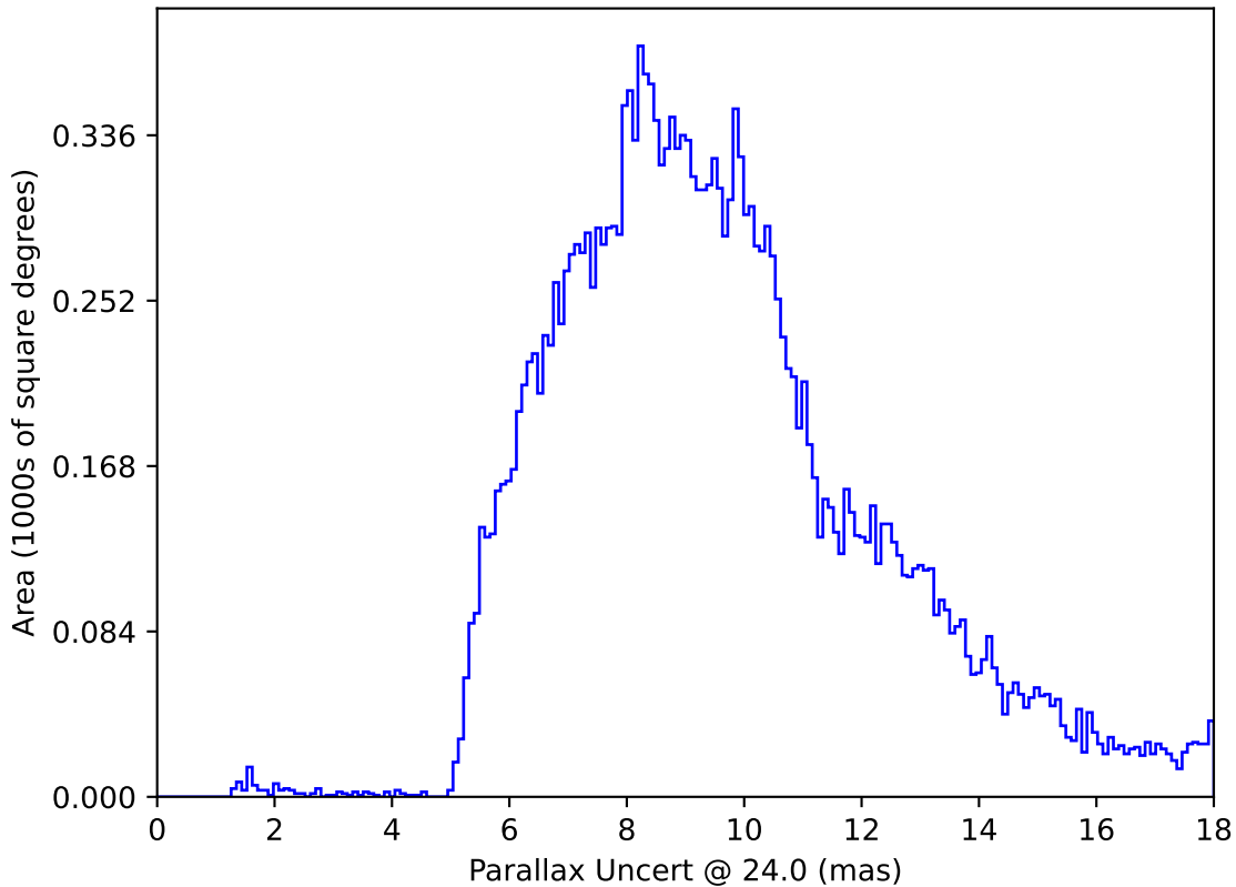
ddf_acor_sf20_lsf40_lsr50_v3.4_10yrs All sky: Parallax Uncert @ 24.0
