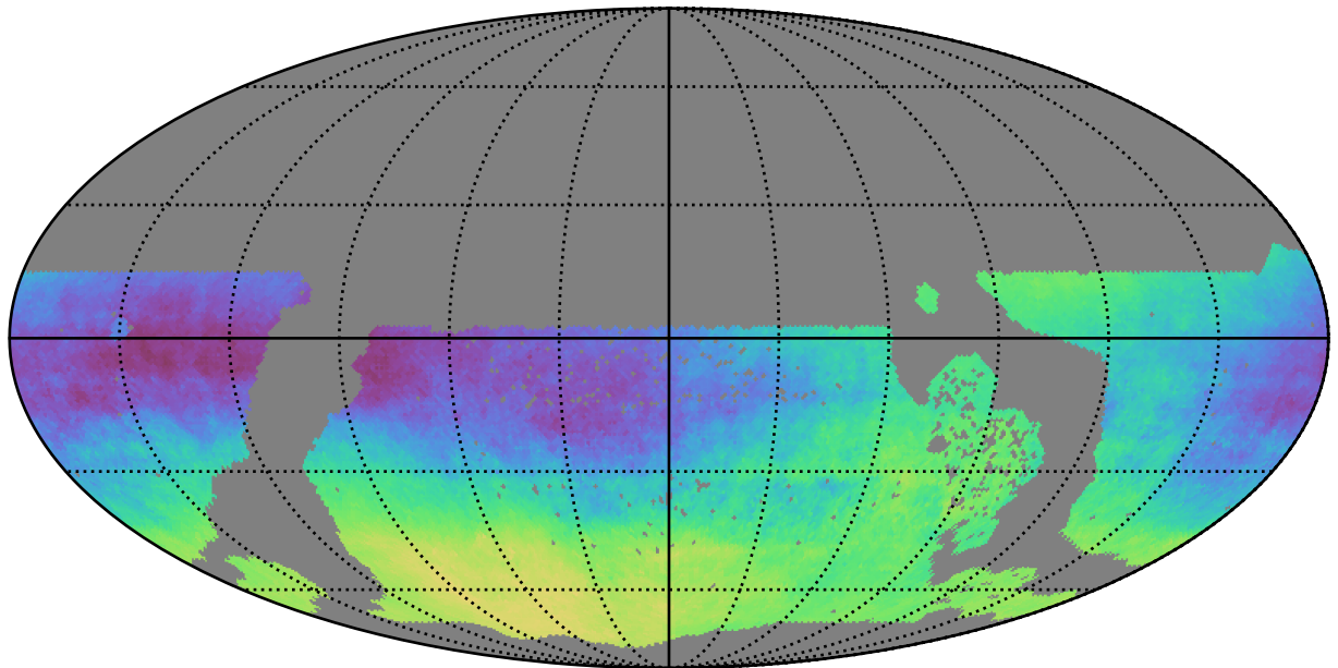
ddf_acor_sf20_lsf40_lsr50_v3.4_10yrs WFD: Parallax-DCR degeneracy @ 24.0
