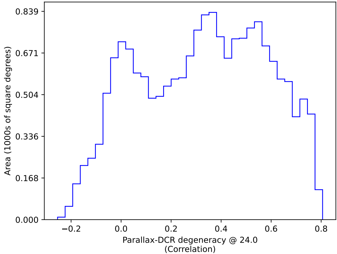
ddf_acor_sf20_lsf40_lsr50_v3.4_10yrs WFD: Parallax-DCR degeneracy @ 24.0
