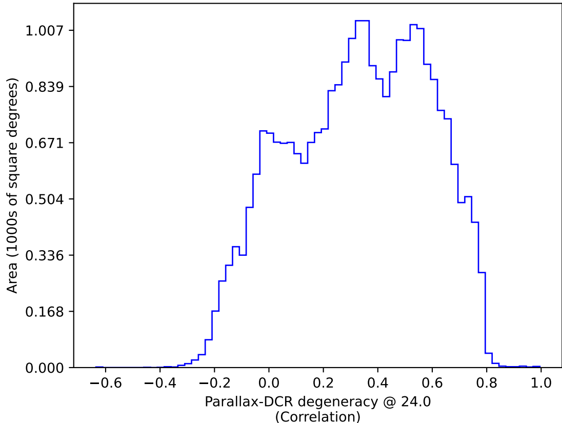
ddf_acor_sf20_lsf40_lsr50_v3.4_10yrs All sky: Parallax-DCR degeneracy @ 24.0
