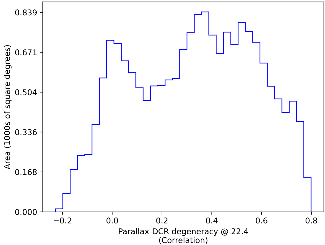
ddf_acor_sf20_lsf40_lsr50_v3.4_10yrs WFD: Parallax-DCR degeneracy @ 22.4
