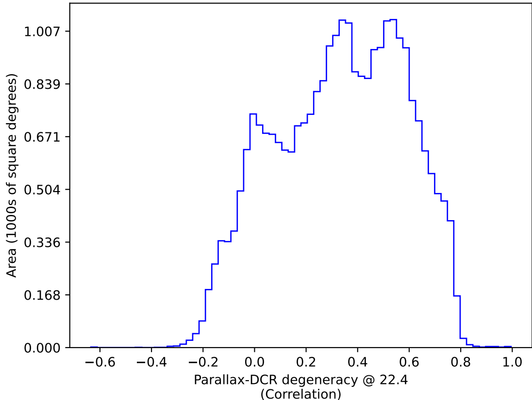
ddf_acor_sf20_lsf40_lsr50_v3.4_10yrs All sky: Parallax-DCR degeneracy @ 22.4
